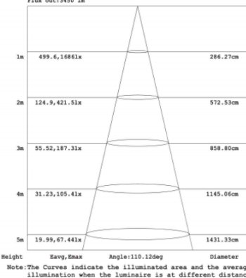
Flux out: 3450 lm
