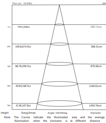
LUMINOUS INTENSITY DISTRIBUTION DIAGRAM
